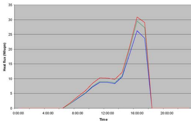
Figure. Surface physical properties of modeled double wall glazing system
