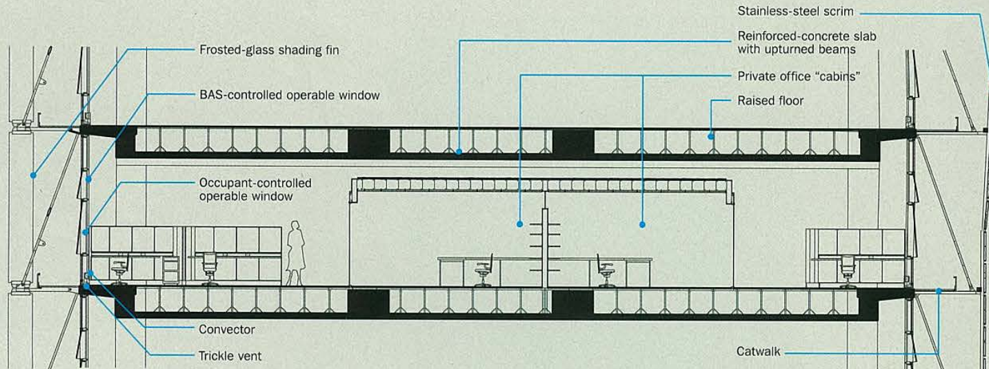
SECTION DETAIL THROUGH TYPICAL OFFICE FLOOR
