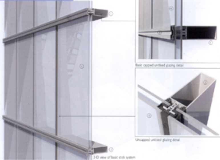
Walls 02 Glass systems: 1: stick systems
