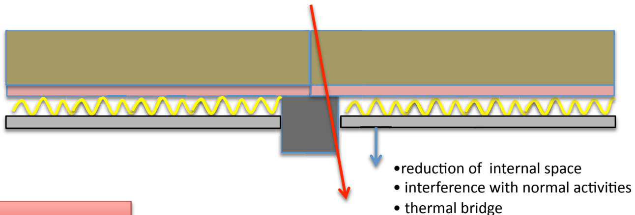
Insulation from inside
