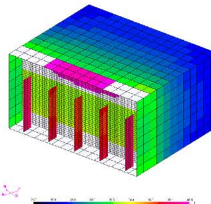
TYPICAL BOX MODEL FOR SOLAR LOADS (RAD-THERM)
